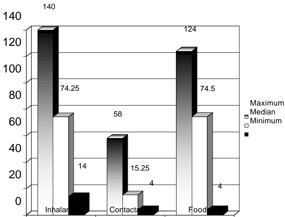
Figure 10: Pre-treatment Antigens Testing Positive Divided by Type of Allergen
