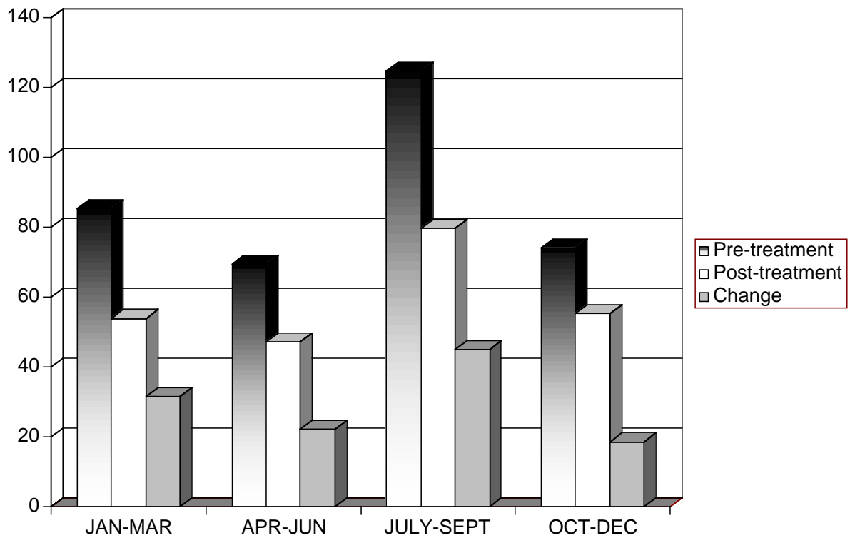
Figure 4: Pre- and Post-treatment Scores by Season
